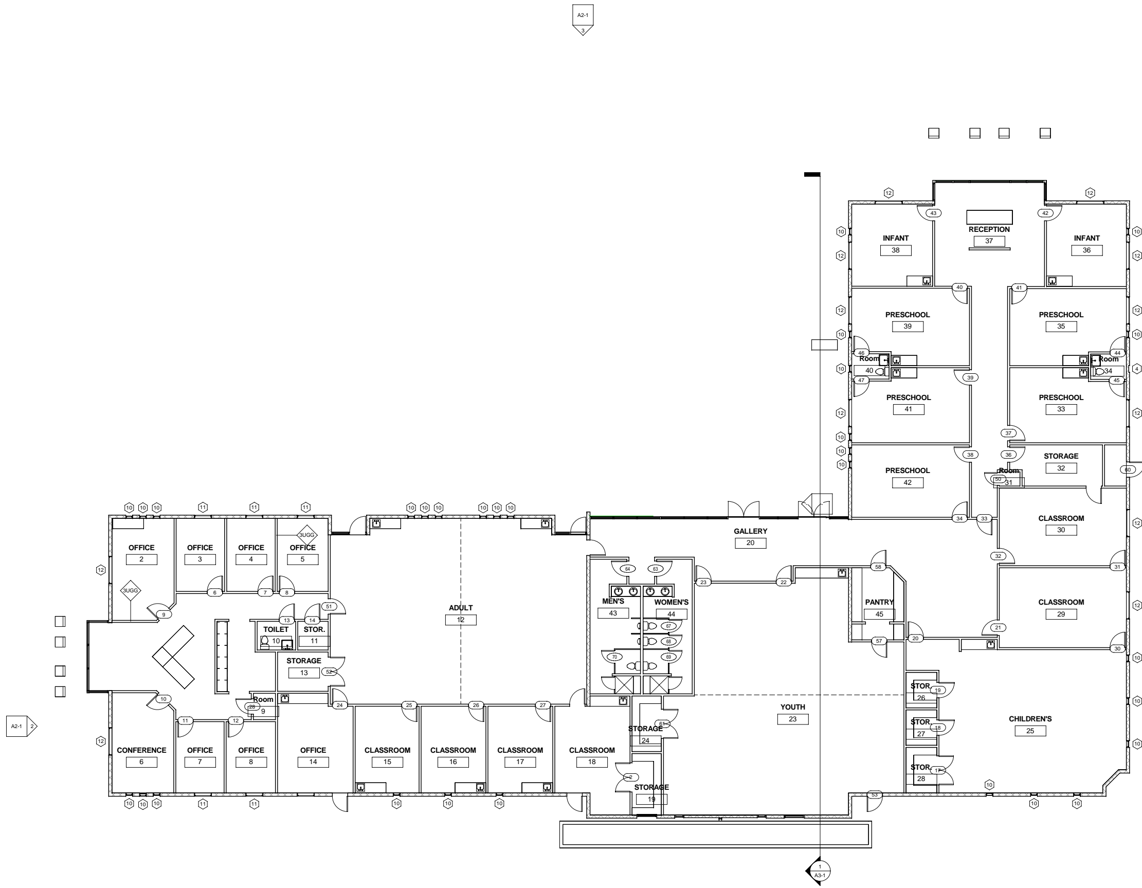
1 Floor Plan 1/8" = 1'-0"
